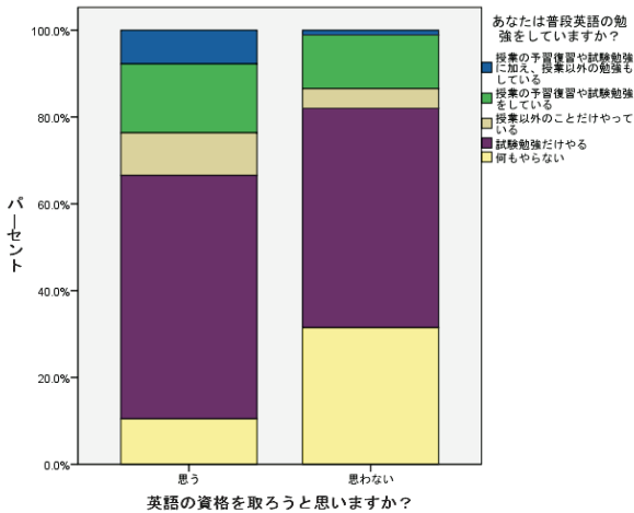
Fig. 6 Correlation between Q17 and Q22
